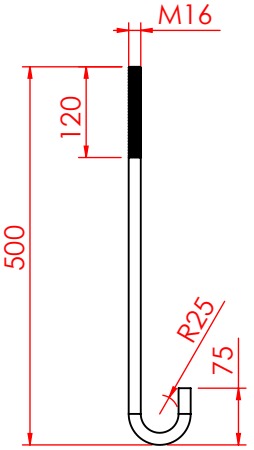
ANCHOR BOLT DETAILS GALVANIZED STEEL
