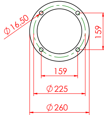
SCALE 1 : 10 t:2mm
