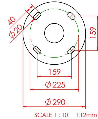
BASE PLATE DETAIL GALVANIZED STEEL
