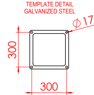
SCALE 1 : 20 t:2mm
