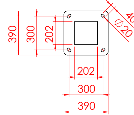
SCALE 1 : 20 t:10mm
