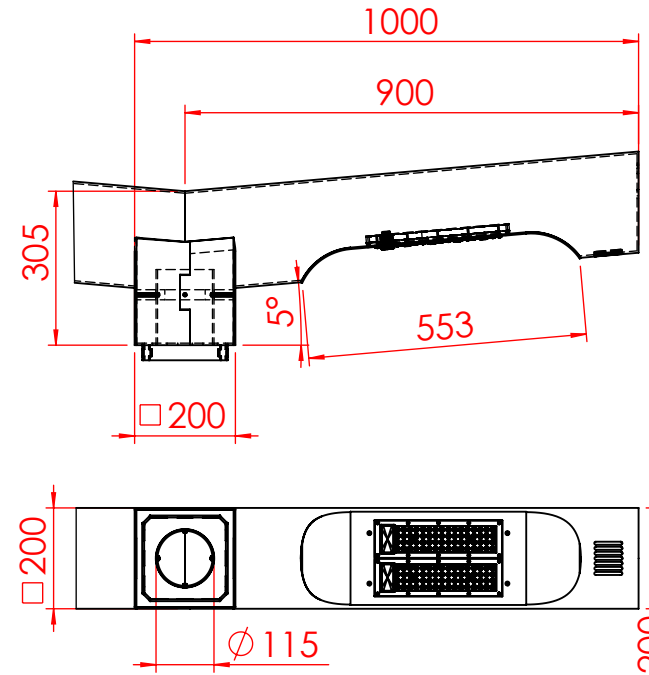
BASE PLATE DETAIL ALUMINUM
