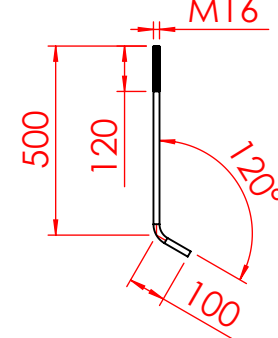
ANCHOR BOLT DETAILS GALVANIZED STEEL
